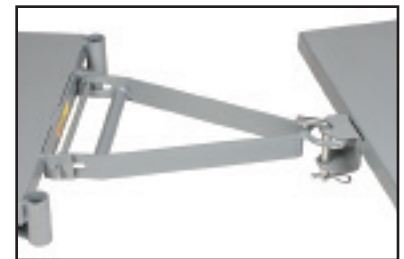
Versatile ring type wishbone coupler with 2-1/2" I.D. Ring can also be used with most pintle hitches.
